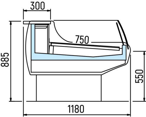
ASPEN 2 SELF FISH
