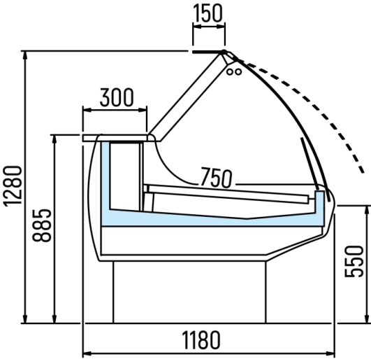
ASPEN 2 VCA FISH
